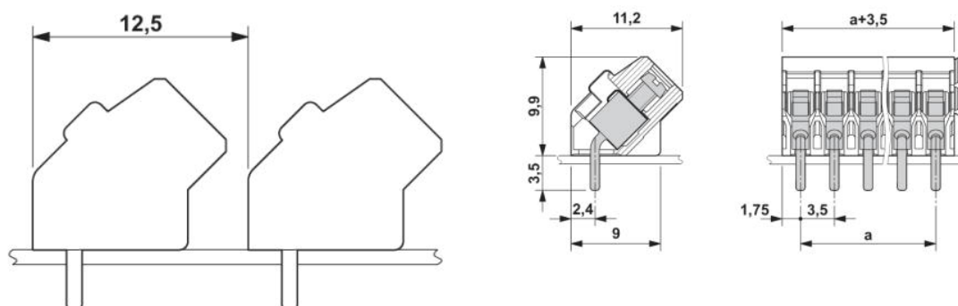
Dimensioned drawing
